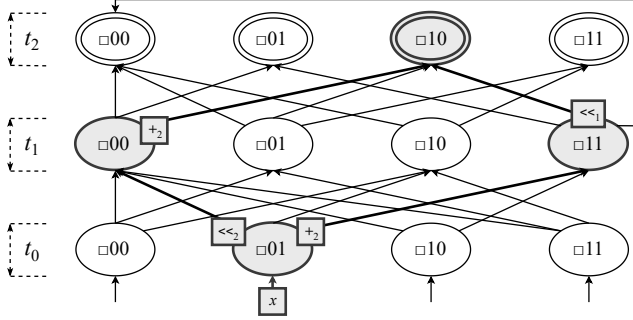
Fig. 3. Offline FTA \mathcal{A} for our DSL using abstract semantics that tracks the lowest two bits. We highlight the part of \mathcal{A} that corresponds to the slice \mathcal{A}_{e_1} for the first example e_1 : \{x = 0001\} \mapsto 0110 , and we elide labels for transitions not in \mathcal{A}_{e_1} to simplify the presentation.
